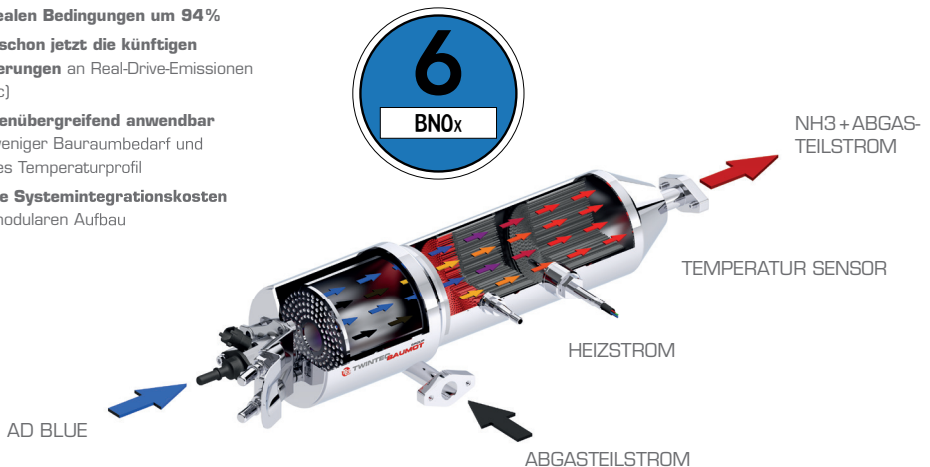
BNOx NH3 Generator
